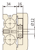
截面BB
